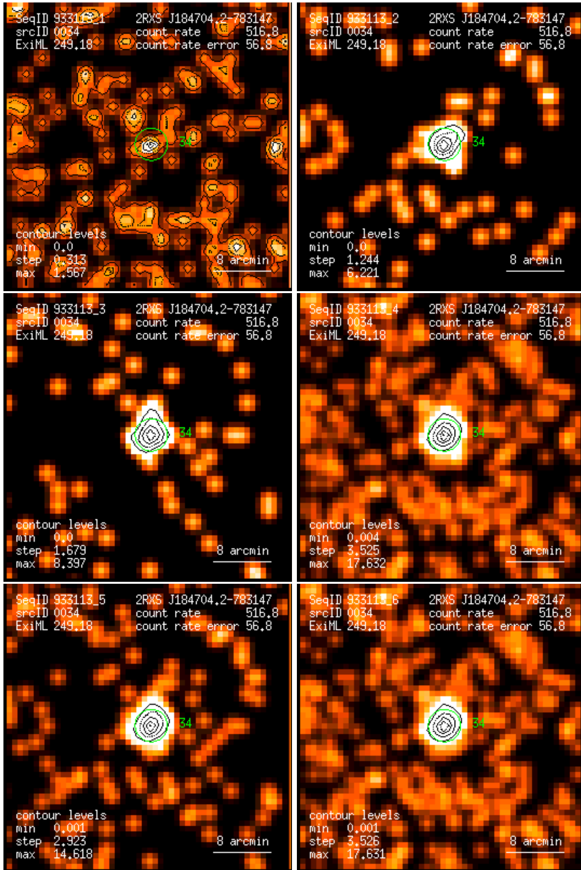
Figure 34: RASS 933113: detection 0034: band rate images, Gaussian filter: (1) PSPC channels 11 – 41, (2) 52 – 90, (3) 91 – 201, (4) 11 – 235, (5) 52 – 201, (6) 11 – 201. Broad band rates in counts/ks. Band rate contour levels in counts/ks/arcmin 2 .
