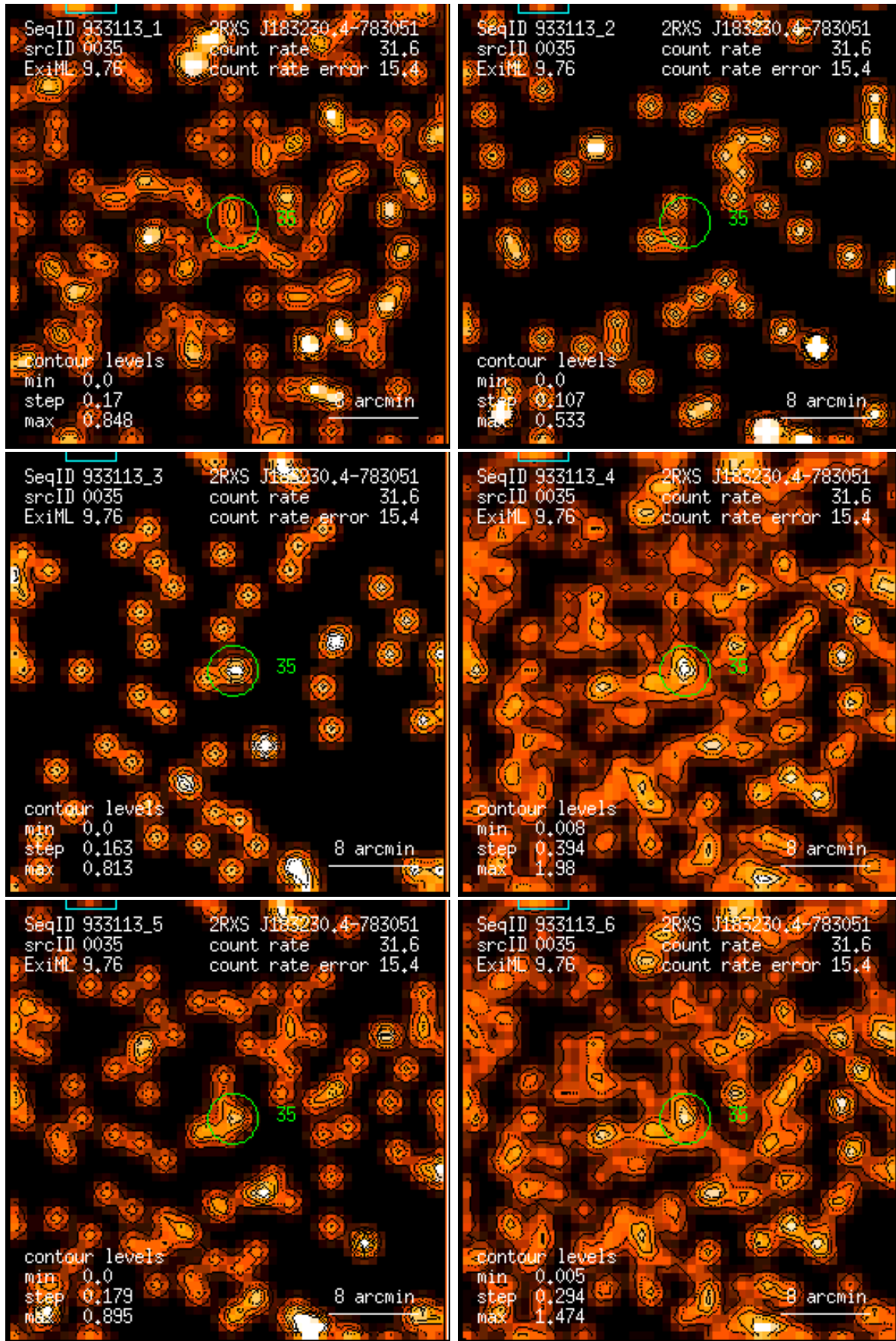
Figure 35: RASS 933113: detection 0035: band rate images, Gaussian filter: (1) PSPC channels 11 – 41, (2) 52 – 90, (3) 91 – 201, (4) 11 – 235, (5) 52 – 201, (6) 11 – 201. Broad band rates in counts/ks. Band rate contour levels in counts/ks/arcmin 2 .
