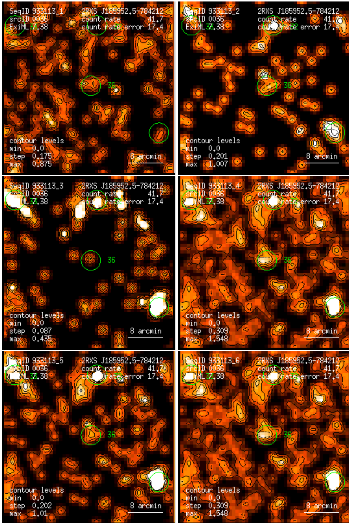
Figure 36: RASS 933113: detection 0036: band rate images, Gaussian filter: (1) PSPC channels 11 – 41, (2) 52 – 90, (3) 91 – 201, (4) 11 – 235, (5) 52 – 201, (6) 11 – 201. Broad band rates in counts/ks. Band rate contour levels in counts/ks/arcmin 2 .
