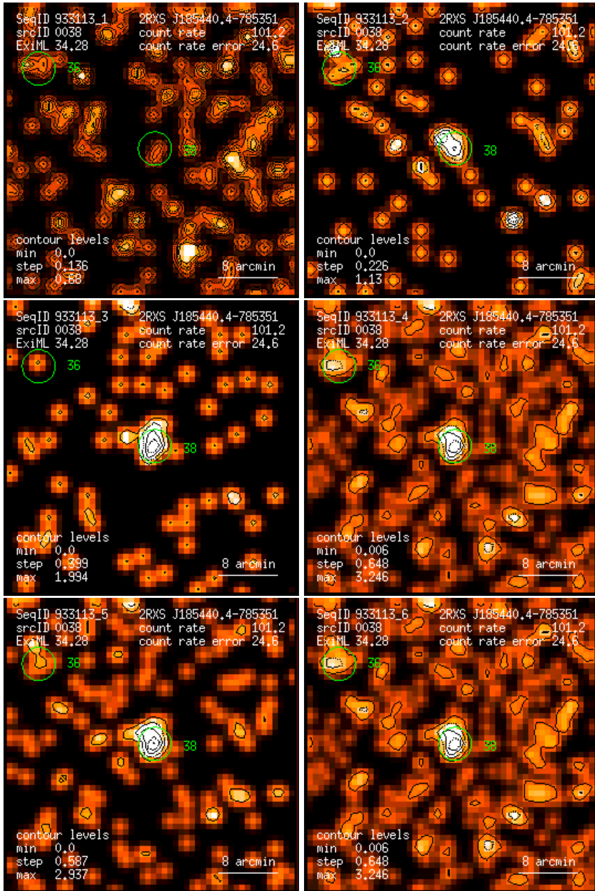
Figure 38: RASS 933113: detection 0038: band rate images, Gaussian filter: (1) PSPC channels 11 – 41, (2) 52 – 90, (3) 91 – 201, (4) 11 – 235, (5) 52 – 201, (6) 11 – 201. Broad band rates in counts/ks. Band rate contour levels in counts/ks/arcmin 2 .
