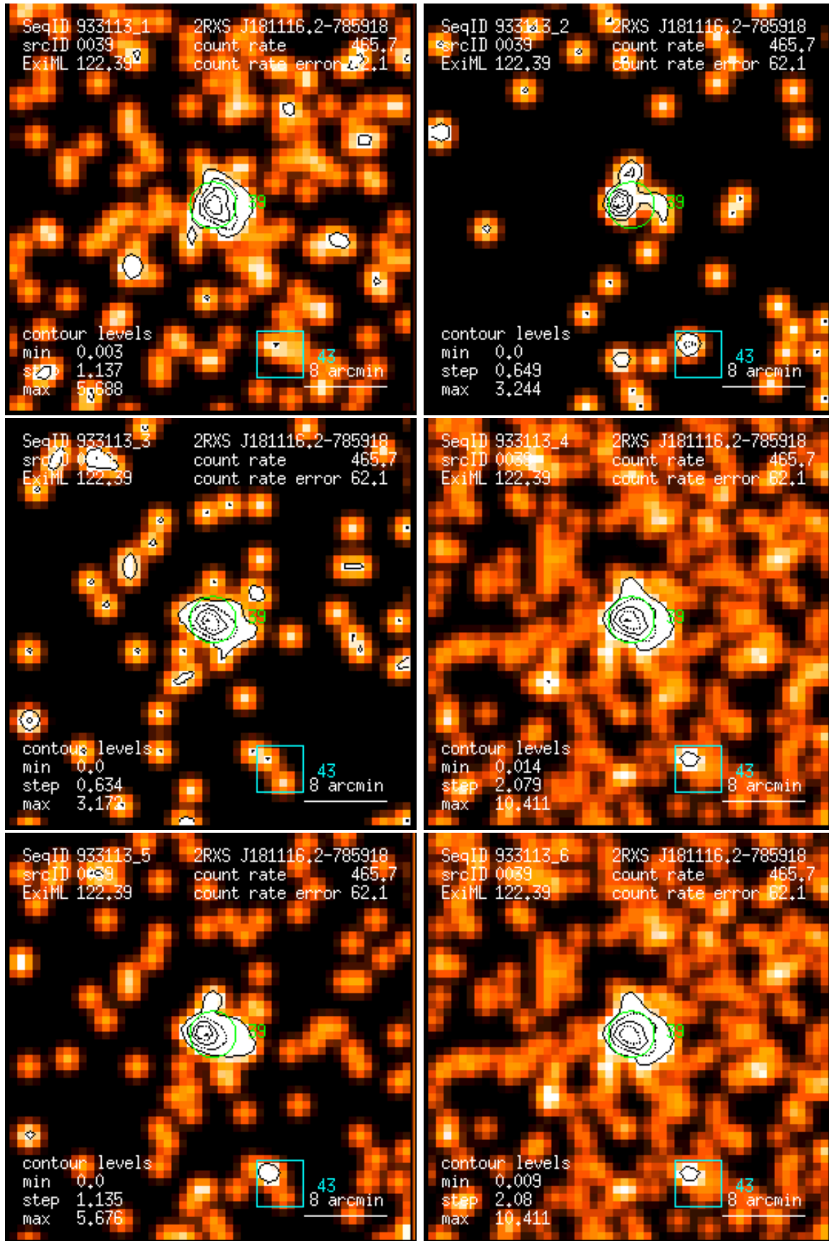
Figure 39: RASS 933113: detection 0039: band rate images, Gaussian filter: (1) PSPC channels 11 – 41, (2) 52 – 90, (3) 91 – 201, (4) 11 – 235, (5) 52 – 201, (6) 11 – 201. Broad band rates in counts/ks. Band rate contour levels in counts/ks/arcmin 2 .
