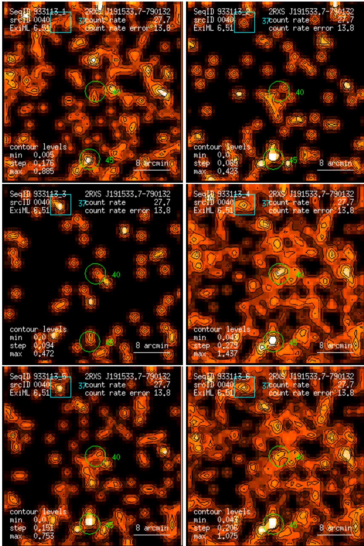
Figure 40: RASS 933113: detection 0040: band rate images, Gaussian filter: (1) PSPC channels 11 – 41, (2) 52 – 90, (3) 91 – 201, (4) 11 – 235, (5) 52 – 201, (6) 11 – 201. Broad band rates in counts/ks. Band rate contour levels in counts/ks/arcmin 2 .
