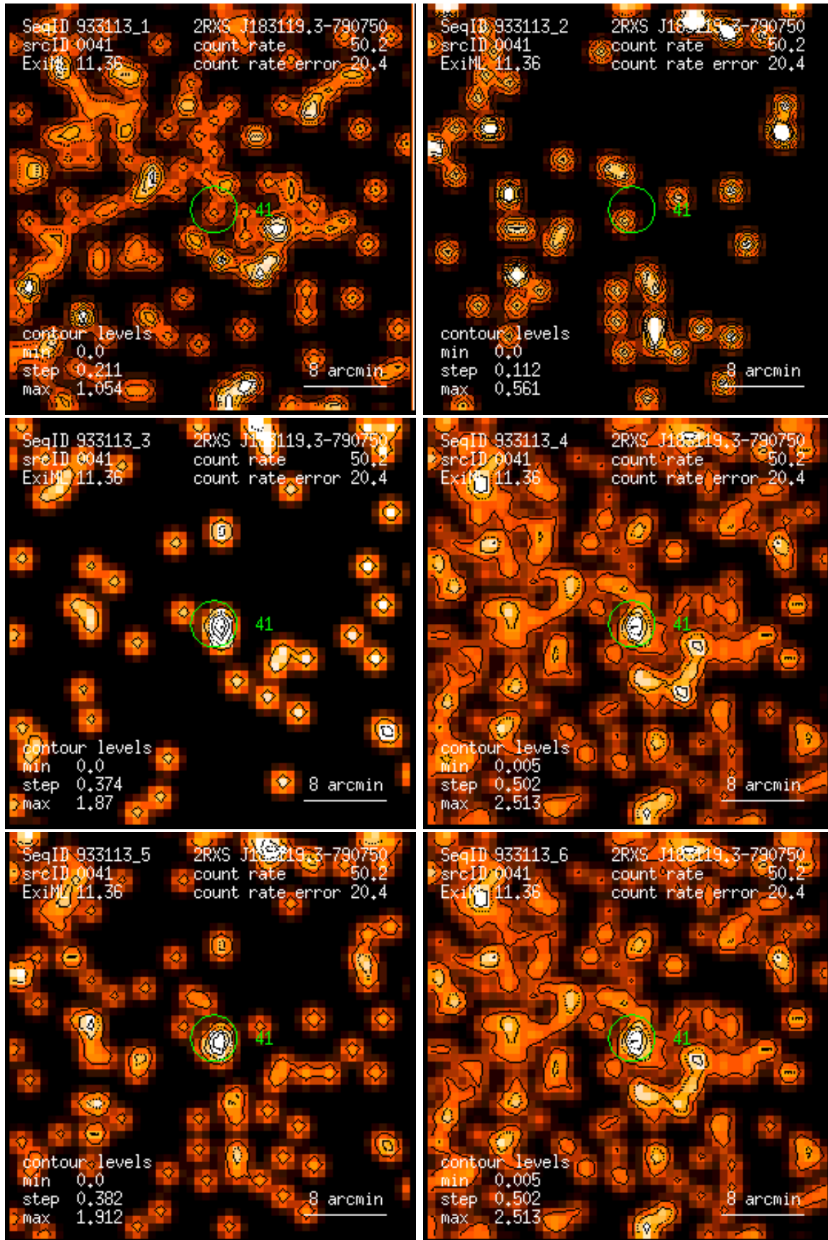
Figure 41: RASS 933113: detection 0041: band rate images, Gaussian filter: (1) PSPC channels 11 – 41, (2) 52 – 90, (3) 91 – 201, (4) 11 – 235, (5) 52 – 201, (6) 11 – 201. Broad band rates in counts/ks. Band rate contour levels in counts/ks/arcmin 2 .
