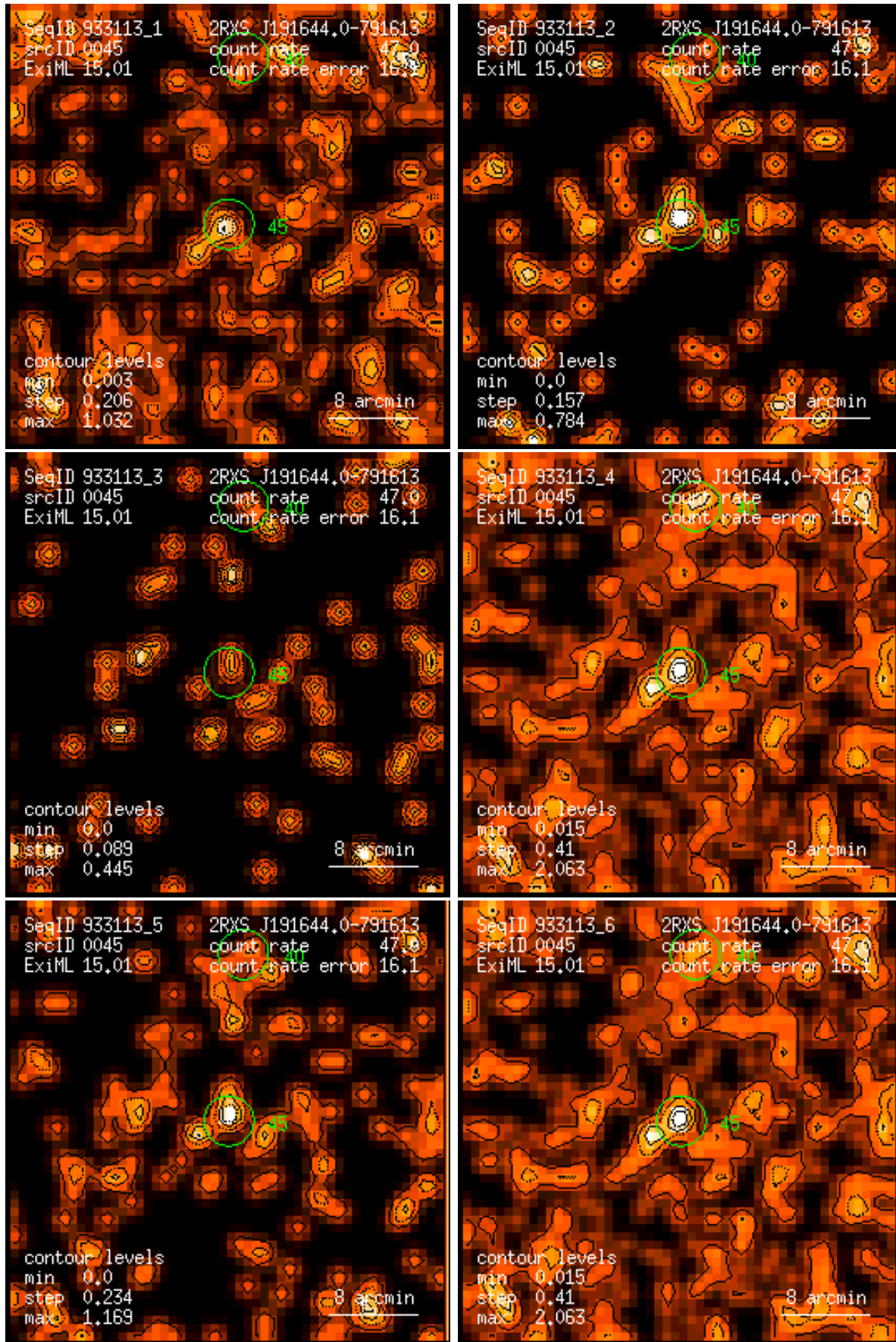
Figure 45: RASS 933113: detection 0045: band rate images, Gaussian filter: (1) PSPC channels 11 – 41, (2) 52 – 90, (3) 91 – 201, (4) 11 – 235, (5) 52 – 201, (6) 11 – 201. Broad band rates in counts/ks. Band rate contour levels in counts/ks/arcmin 2 .
