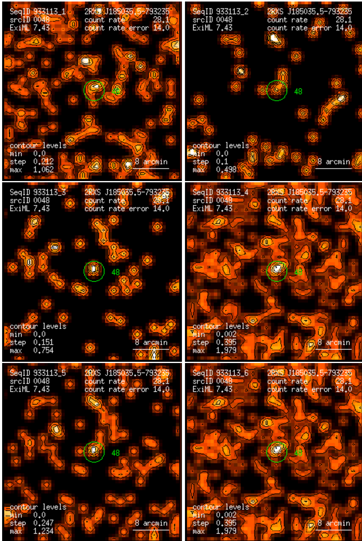
Figure 48: RASS 933113: detection 0048: band rate images, Gaussian filter: (1) PSPC channels 11 – 41, (2) 52 – 90, (3) 91 – 201, (4) 11 – 235, (5) 52 – 201, (6) 11 – 201. Broad band rates in counts/ks. Band rate contour levels in counts/ks/arcmin 2 .
