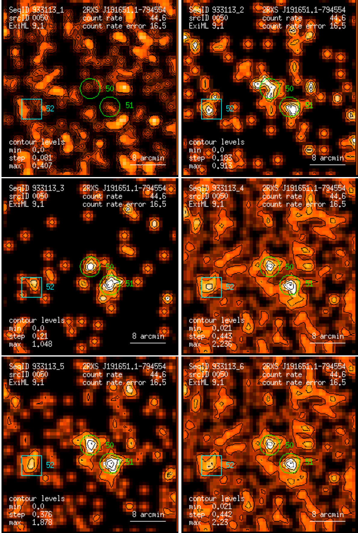
Figure 50: RASS 933113: detection 0050: band rate images, Gaussian filter: (1) PSPC channels 11 – 41, (2) 52 – 90, (3) 91 – 201, (4) 11 – 235, (5) 52 – 201, (6) 11 – 201. Broad band rates in counts/ks. Band rate contour levels in counts/ks/arcmin 2 .
