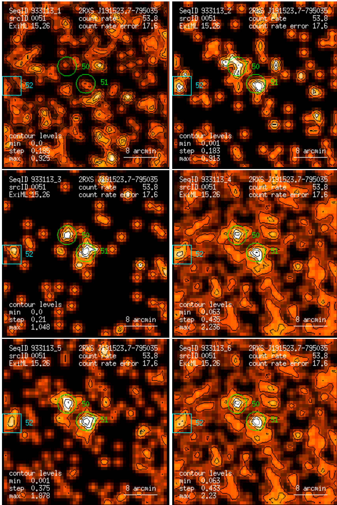
Figure 51: RASS 933113: detection 0051: band rate images, Gaussian filter: (1) PSPC channels 11 – 41, (2) 52 – 90, (3) 91 – 201, (4) 11 – 235, (5) 52 – 201, (6) 11 – 201. Broad band rates in counts/ks. Band rate contour levels in counts/ks/arcmin 2 .
