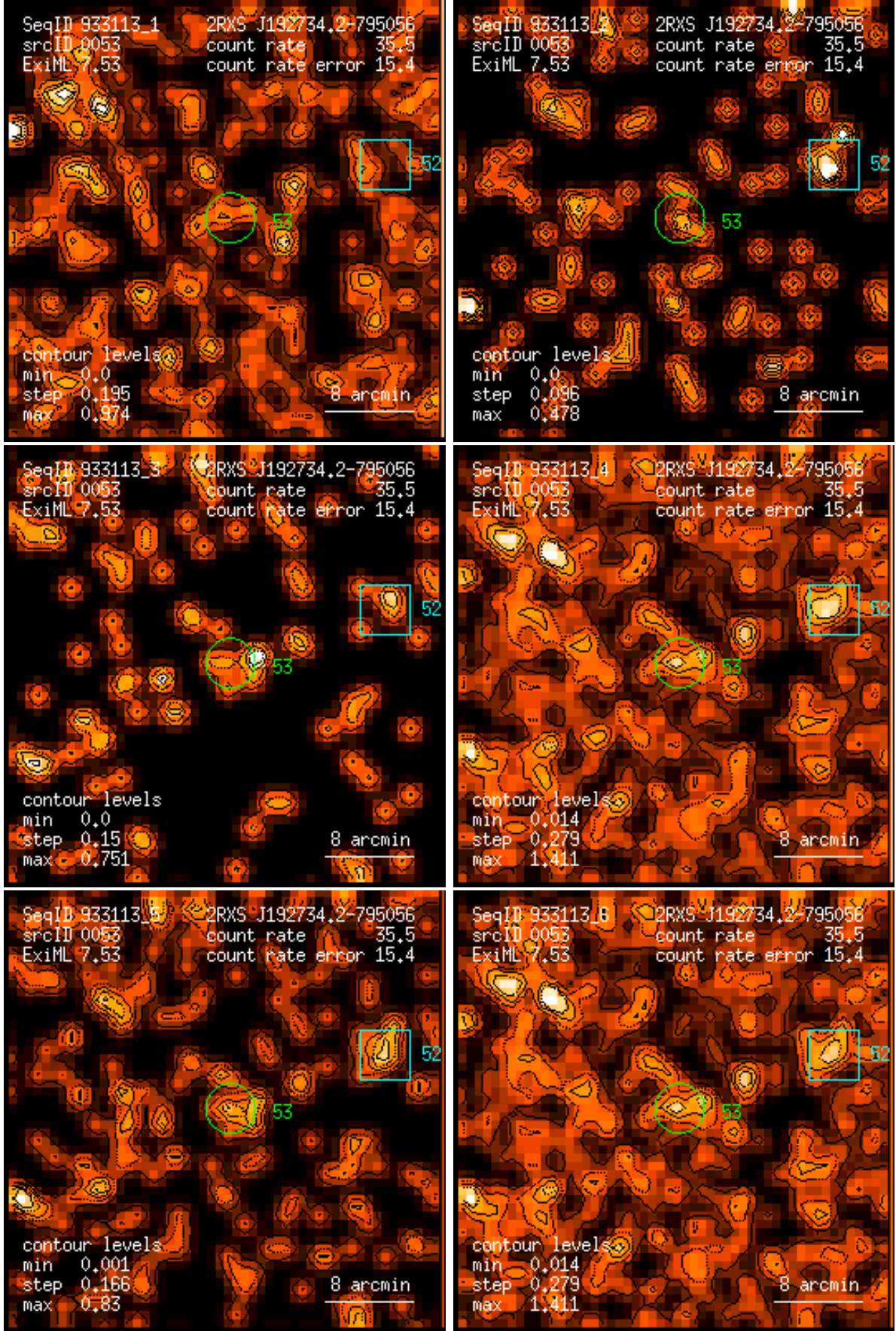
Figure 53: RASS 933113: detection 0053: band rate images, Gaussian filter: (1) PSPC channels 11 – 41, (2) 52 – 90, (3) 91 – 201, (4) 11 – 235, (5) 52 – 201, (6) 11 – 201. Broad band rates in counts/ks. Band rate contour levels in counts/ks/arcmin 2 .
