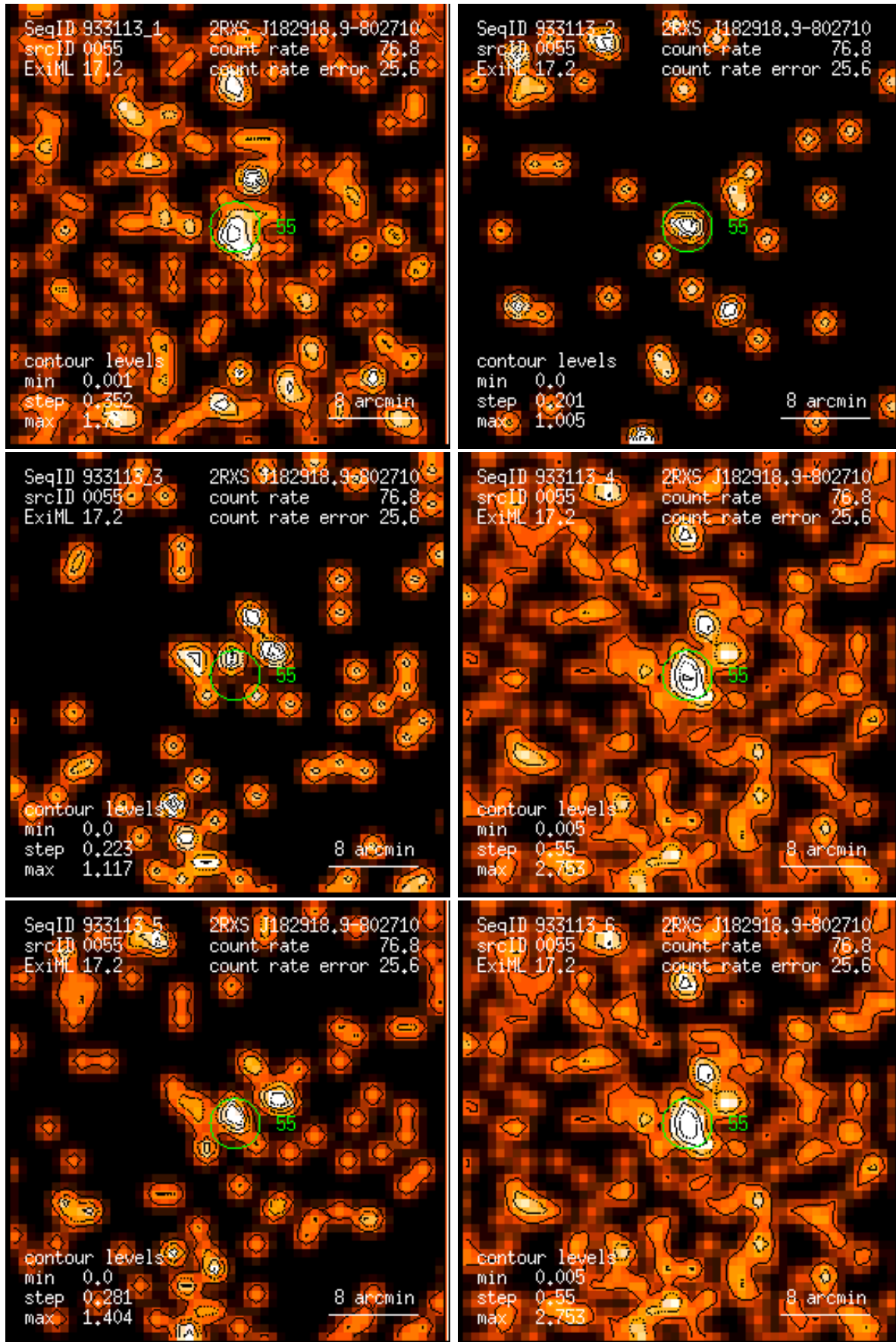
Figure 55: RASS 933113: detection 0055: band rate images, Gaussian filter: (1) PSPC channels 11 – 41, (2) 52 – 90, (3) 91 – 201, (4) 11 – 235, (5) 52 – 201, (6) 11 – 201. Broad band rates in counts/ks. Band rate contour levels in counts/ks/arcmin 2 .
