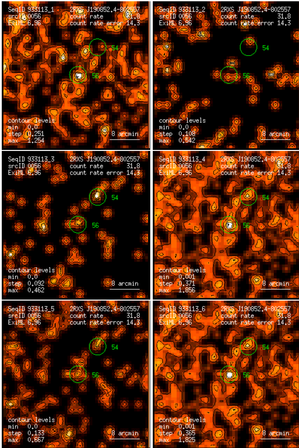
Figure 56: RASS 933113: detection 0056: band rate images, Gaussian filter: (1) PSPC channels 11 – 41, (2) 52 – 90, (3) 91 – 201, (4) 11 – 235, (5) 52 – 201, (6) 11 – 201. Broad band rates in counts/ks. Band rate contour levels in counts/ks/arcmin 2 .
