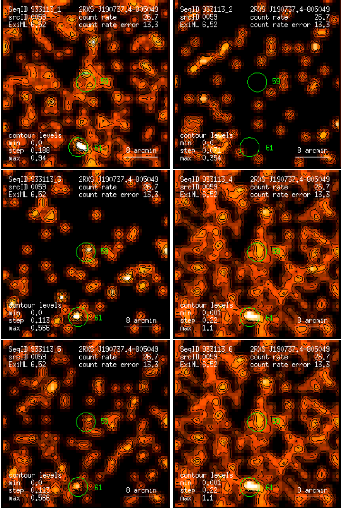
Figure 59: RASS 933113: detection 0059: band rate images, Gaussian filter: (1) PSPC channels 11 – 41, (2) 52 – 90, (3) 91 – 201, (4) 11 – 235, (5) 52 – 201, (6) 11 – 201. Broad band rates in counts/ks. Band rate contour levels in counts/ks/arcmin 2 .
