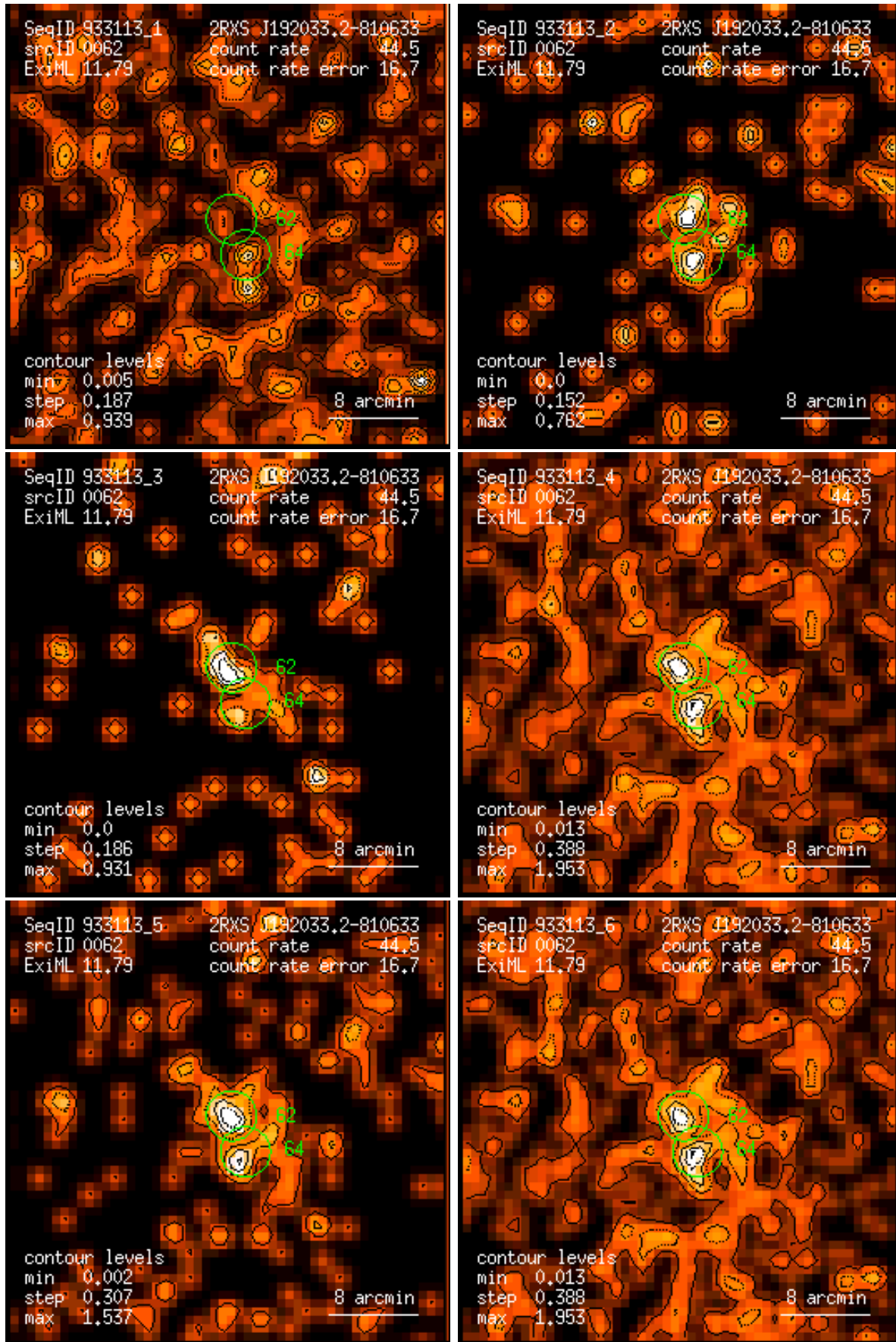
Figure 62: RASS 933113: detection 0062: band rate images, Gaussian filter: (1) PSPC channels 11 – 41, (2) 52 – 90, (3) 91 – 201, (4) 11 – 235, (5) 52 – 201, (6) 11 – 201. Broad band rates in counts/ks. Band rate contour levels in counts/ks/arcmin 2 .
