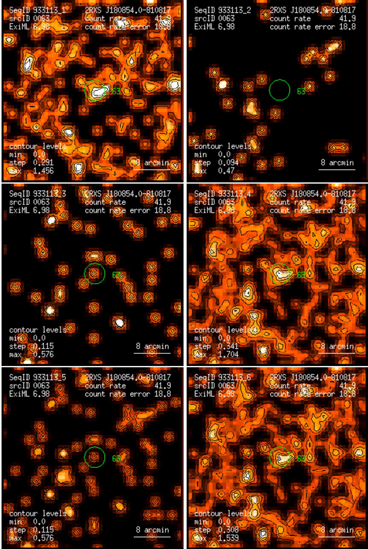
Figure 63: RASS 933113: detection 0063: band rate images, Gaussian filter: (1) PSPC channels 11 – 41, (2) 52 – 90, (3) 91 – 201, (4) 11 – 235, (5) 52 – 201, (6) 11 – 201. Broad band rates in counts/ks. Band rate contour levels in counts/ks/arcmin 2 .
