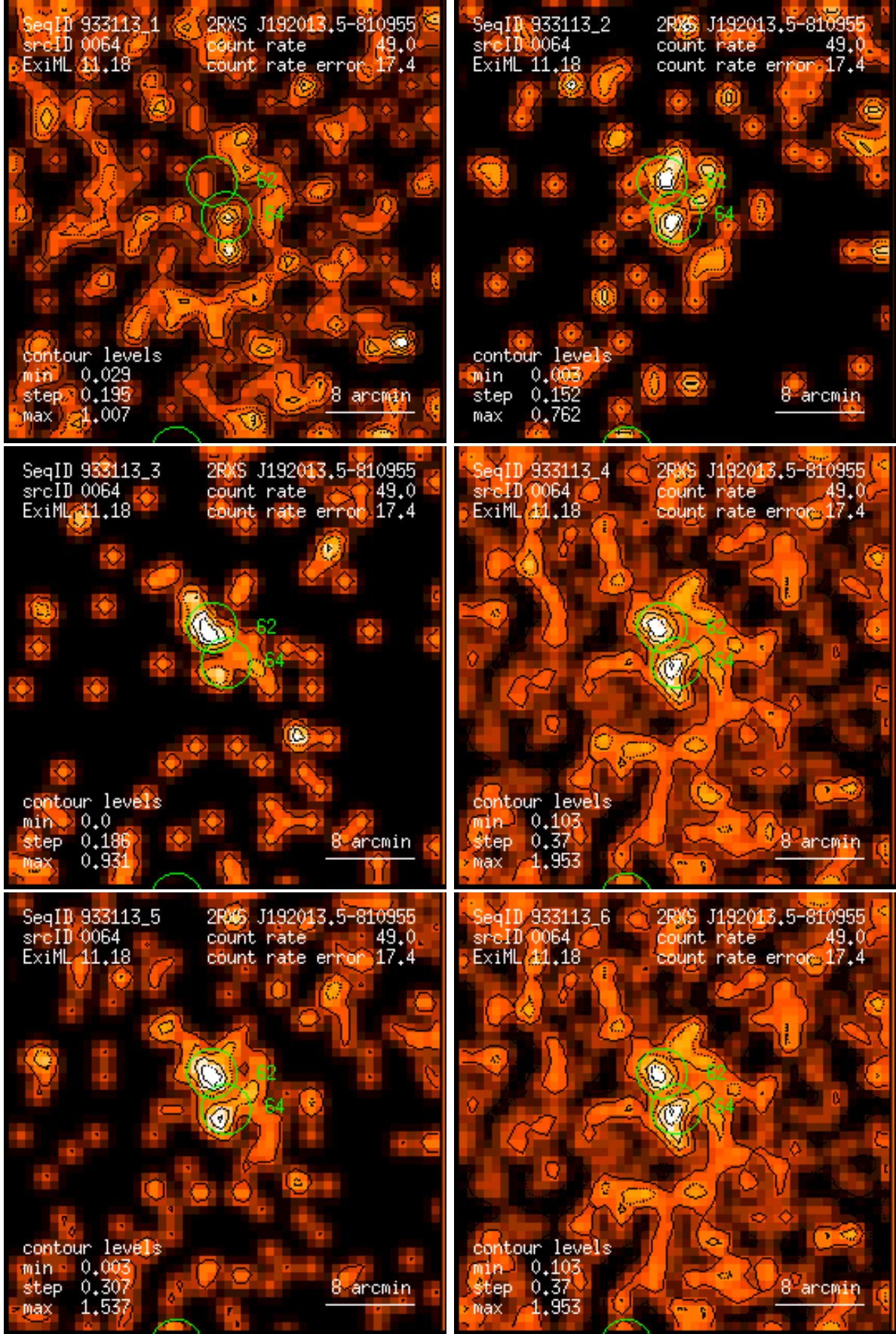
Figure 64: RASS 933113: detection 0064: band rate images, Gaussian filter: (1) PSPC channels 11 – 41, (2) 52 – 90, (3) 91 – 201, (4) 11 – 235, (5) 52 – 201, (6) 11 – 201. Broad band rates in counts/ks. Band rate contour levels in counts/ks/arcmin 2 .
