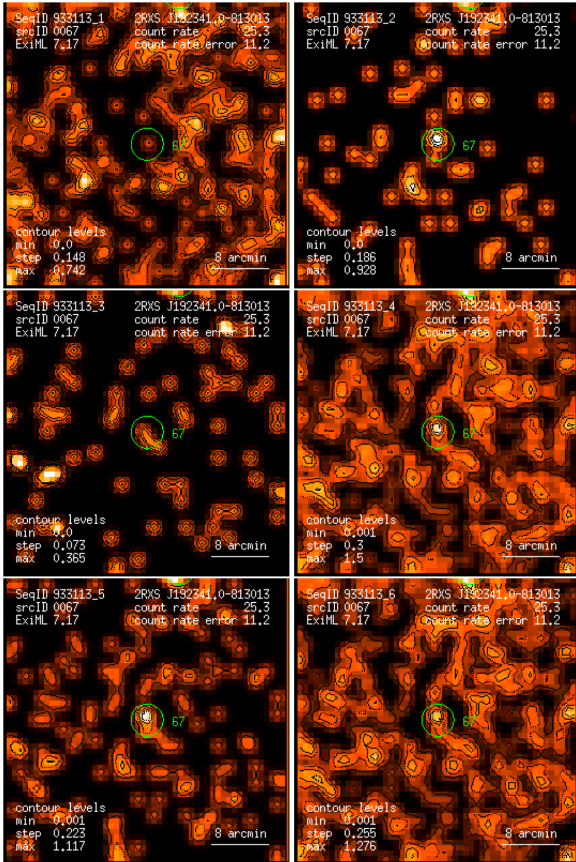
Figure 67: RASS 933113: detection 0067: band rate images, Gaussian filter: (1) PSPC channels 11 – 41, (2) 52 – 90, (3) 91 – 201, (4) 11 – 235, (5) 52 – 201, (6) 11 – 201. Broad band rates in counts/ks. Band rate contour levels in counts/ks/arcmin 2 .
