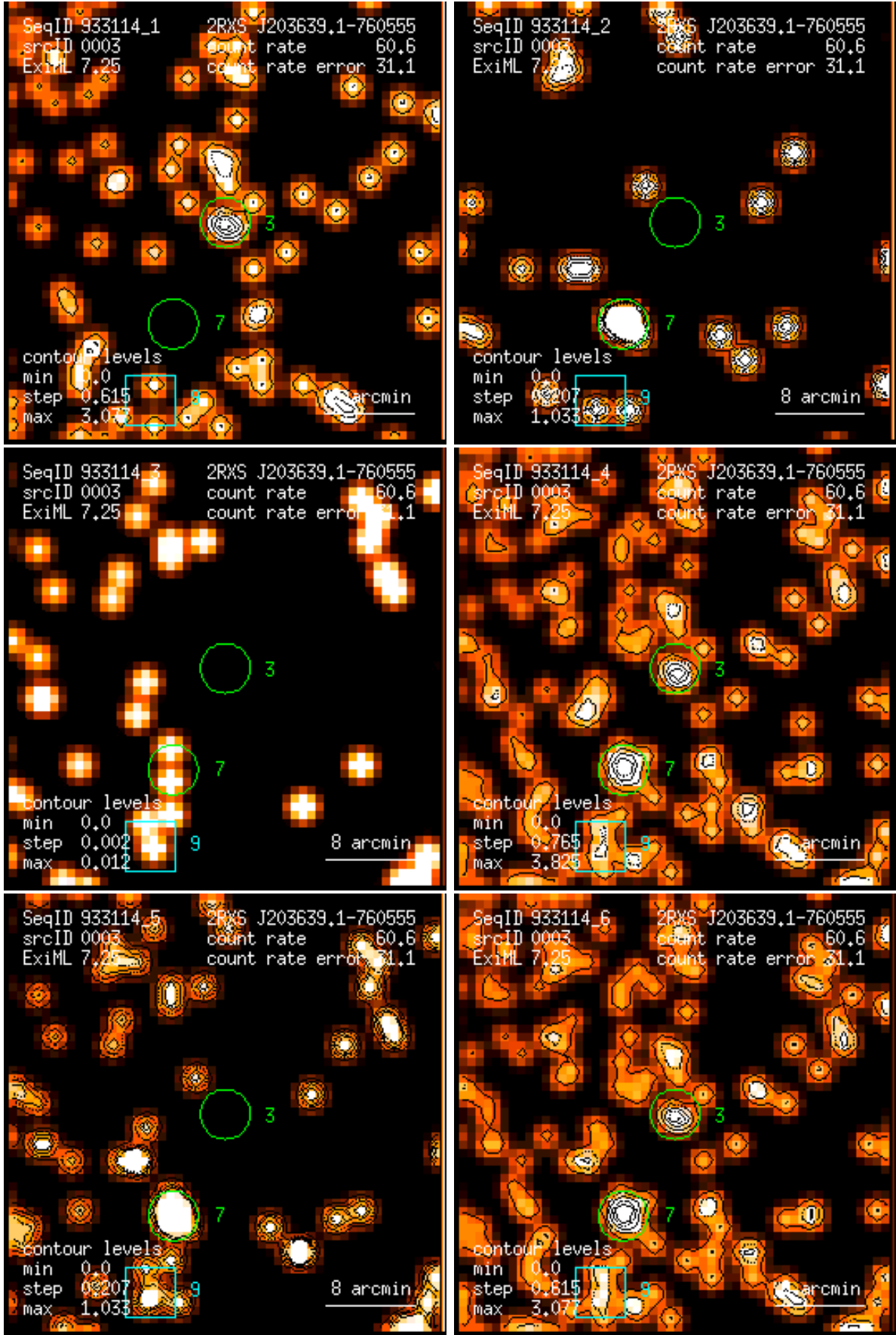
Figure 3: RASS 933114: detection 0003: band rate images, Gaussian filter: (1) PSPC channels 11 – 41, (2) 52 – 90, (3) 91 – 201, (4) 11 – 235, (5) 52 – 201, (6) 11 – 201. Broad band rates in counts/ks. Band rate contour levels in counts/ks/arcmin 2 .
