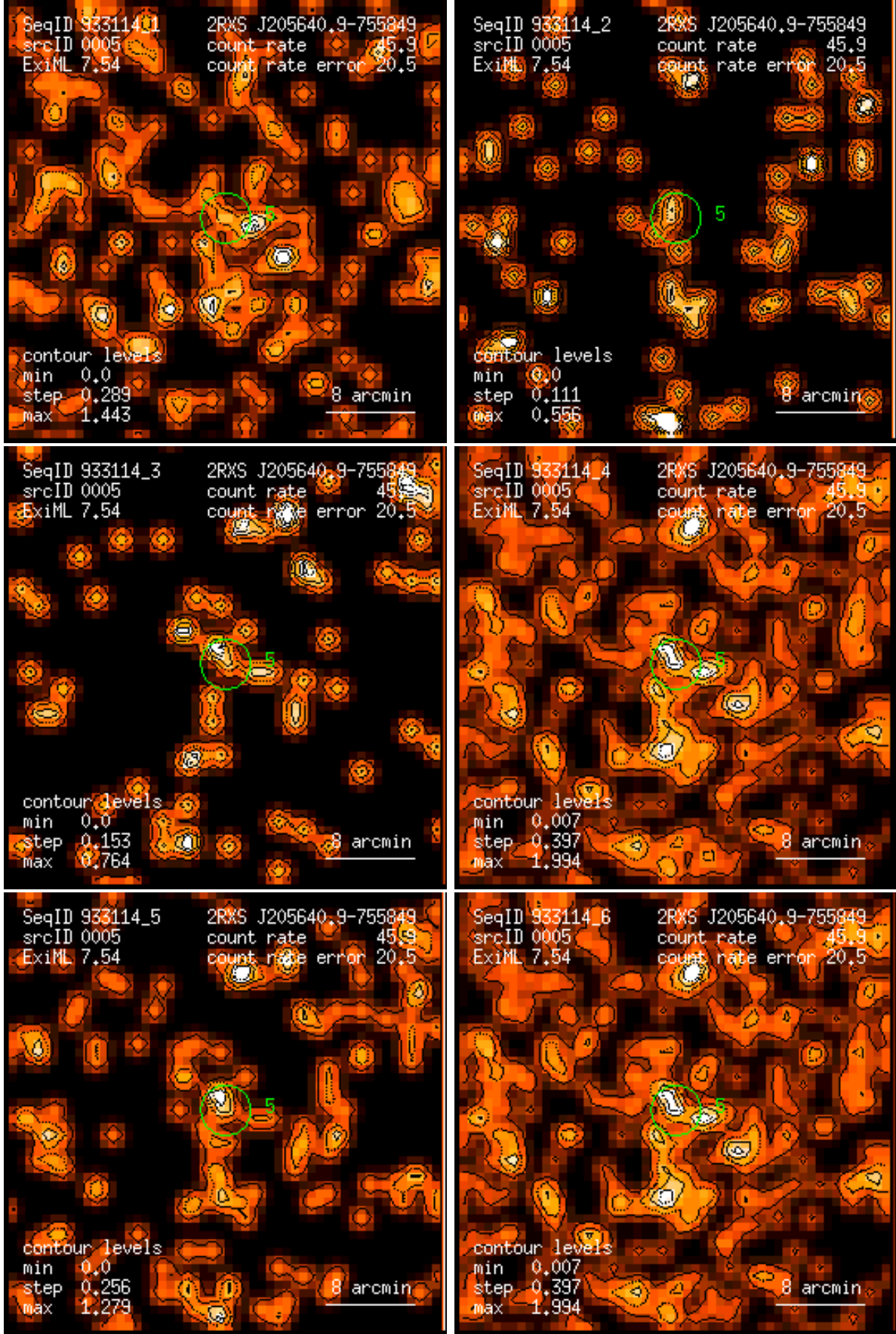
Figure 5: RASS 933114: detection 0005: band rate images, Gaussian filter: (1) PSPC channels 11 – 41, (2) 52 – 90, (3) 91 – 201, (4) 11 – 235, (5) 52 – 201, (6) 11 – 201. Broad band rates in counts/ks. Band rate contour levels in counts/ks/arcmin 2 .
