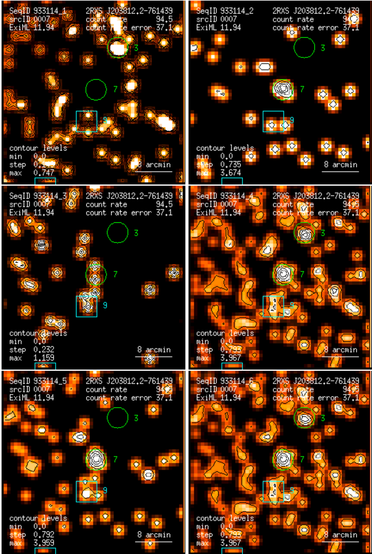
Figure 7: RASS 933114: detection 0007: band rate images, Gaussian filter: (1) PSPC channels 11 – 41, (2) 52 – 90, (3) 91 – 201, (4) 11 – 235, (5) 52 – 201, (6) 11 – 201. Broad band rates in counts/ks. Band rate contour levels in counts/ks/arcmin 2 .
