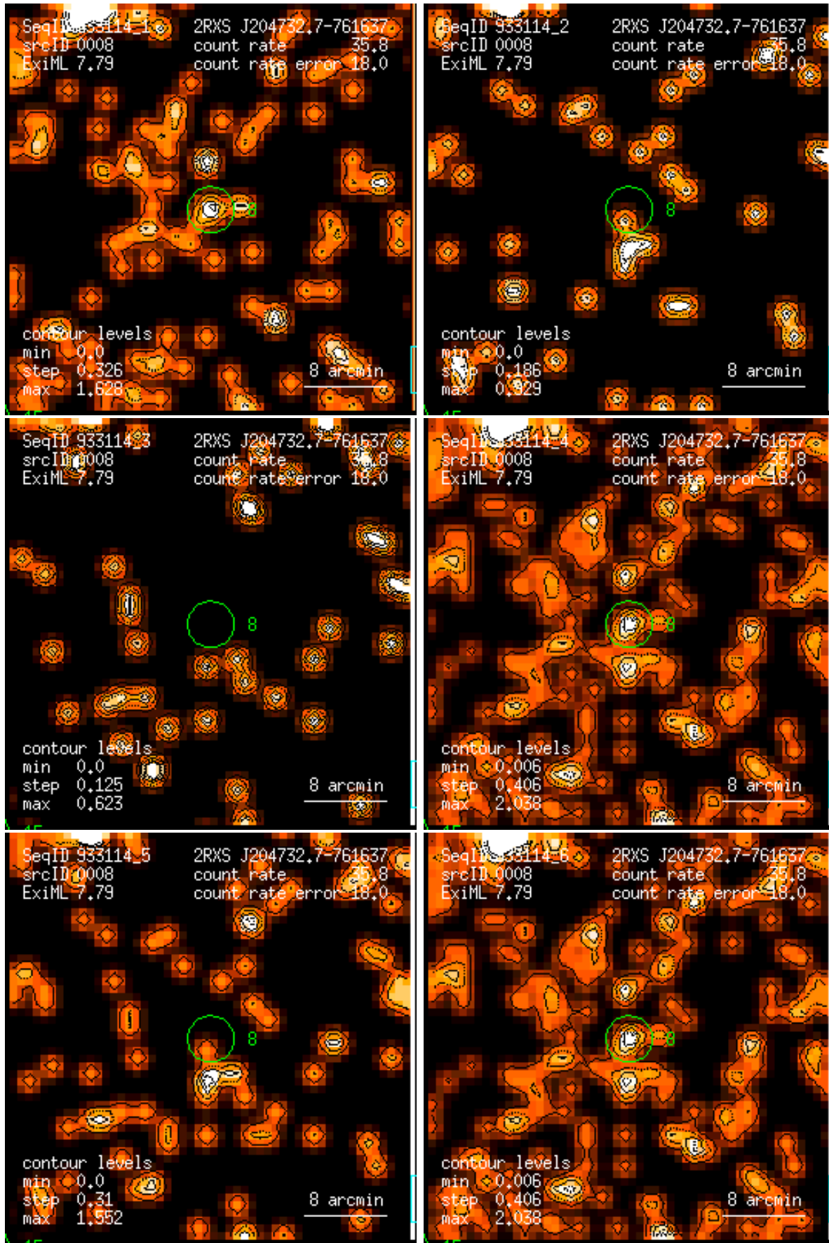
Figure 8: RASS 933114: detection 0008: band rate images, Gaussian filter: (1) PSPC channels 11 – 41, (2) 52 – 90, (3) 91 – 201, (4) 11 – 235, (5) 52 – 201, (6) 11 – 201. Broad band rates in counts/ks. Band rate contour levels in counts/ks/arcmin 2 .
