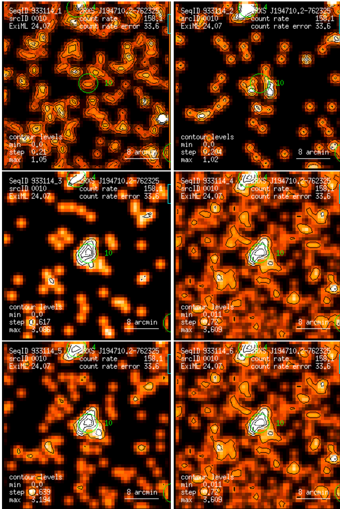
Figure 10: RASS 933114: detection 0010: band rate images, Gaussian filter: (1) PSPC channels 11 – 41, (2) 52 – 90, (3) 91 – 201, (4) 11 – 235, (5) 52 – 201, (6) 11 – 201. Broad band rates in counts/ks. Band rate contour levels in counts/ks/arcmin 2 .
