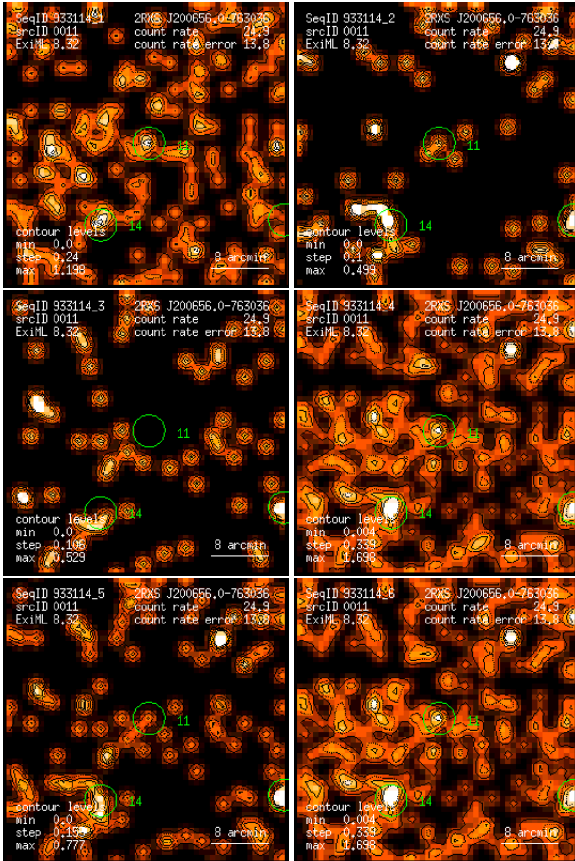
Figure 11: RASS 933114: detection 0011: band rate images, Gaussian filter: (1) PSPC channels 11 – 41, (2) 52 – 90, (3) 91 – 201, (4) 11 – 235, (5) 52 – 201, (6) 11 – 201. Broad band rates in counts/ks. Band rate contour levels in counts/ks/arcmin 2 .
