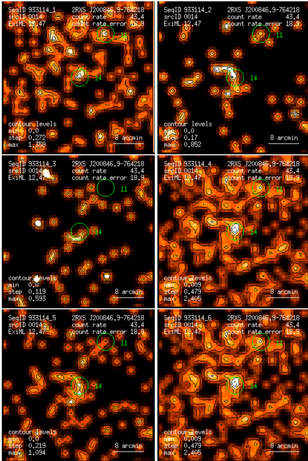
Figure 14: RASS 933114: detection 0014: band rate images, Gaussian filter: (1) PSPC channels 11 – 41, (2) 52 – 90, (3) 91 – 201, (4) 11 – 235, (5) 52 – 201, (6) 11 – 201. Broad band rates in counts/ks. Band rate contour levels in counts/ks/arcmin 2 .
