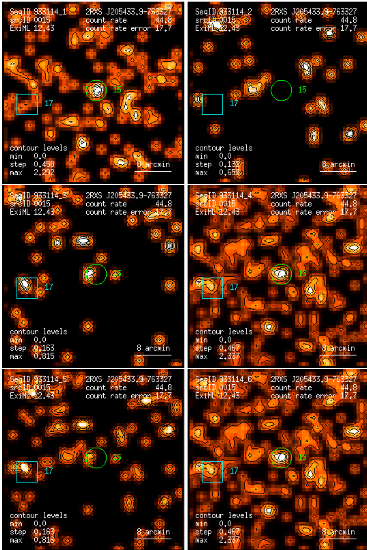
Figure 15: RASS 933114: detection 0015: band rate images, Gaussian filter: (1) PSPC channels 11 – 41, (2) 52 – 90, (3) 91 – 201, (4) 11 – 235, (5) 52 – 201, (6) 11 – 201. Broad band rates in counts/ks. Band rate contour levels in counts/ks/arcmin 2 .
