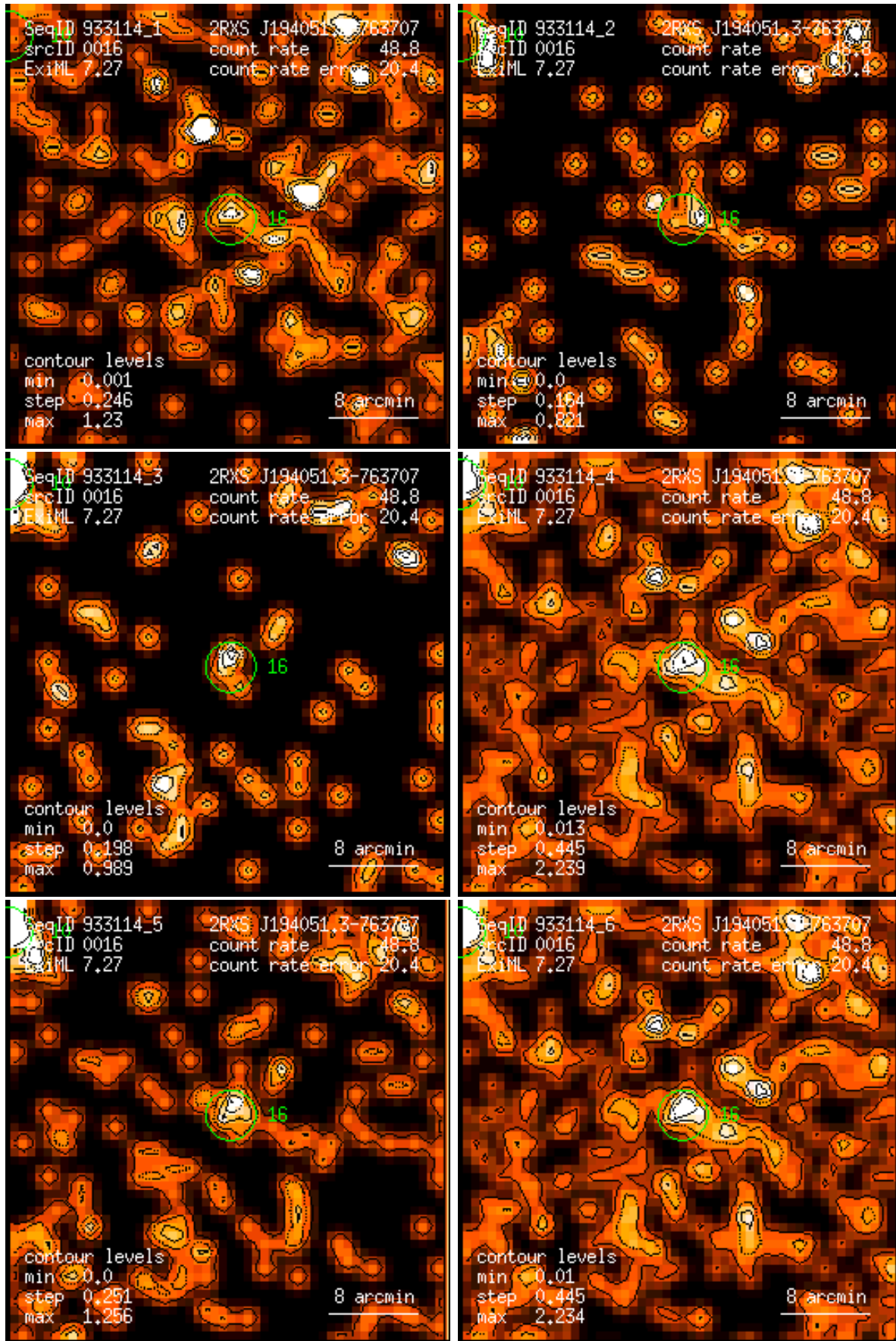
Figure 16: RASS 933114: detection 0016: band rate images, Gaussian filter: (1) PSPC channels 11 – 41, (2) 52 – 90, (3) 91 – 201, (4) 11 – 235, (5) 52 – 201, (6) 11 – 201. Broad band rates in counts/ks. Band rate contour levels in counts/ks/arcmin 2 .
