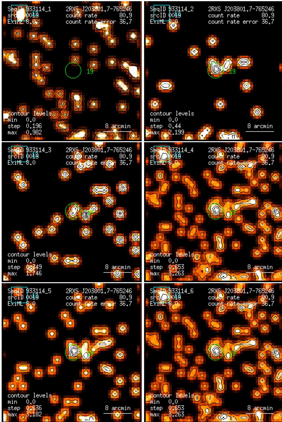
Figure 19: RASS 933114: detection 0019: band rate images, Gaussian filter: (1) PSPC channels 11 – 41, (2) 52 – 90, (3) 91 – 201, (4) 11 – 235, (5) 52 – 201, (6) 11 – 201. Broad band rates in counts/ks. Band rate contour levels in counts/ks/arcmin 2 .
