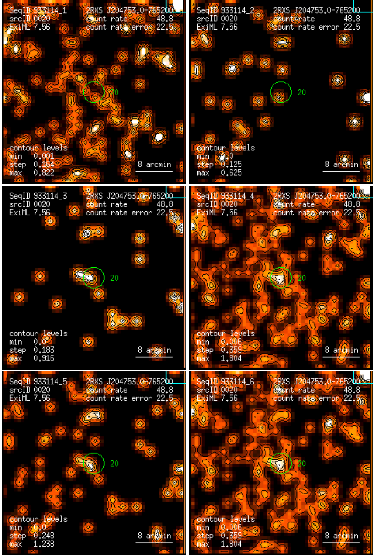
Figure 20: RASS 933114: detection 0020: band rate images, Gaussian filter: (1) PSPC channels 11 – 41, (2) 52 – 90, (3) 91 – 201, (4) 11 – 235, (5) 52 – 201, (6) 11 – 201. Broad band rates in counts/ks. Band rate contour levels in counts/ks/arcmin 2 .
