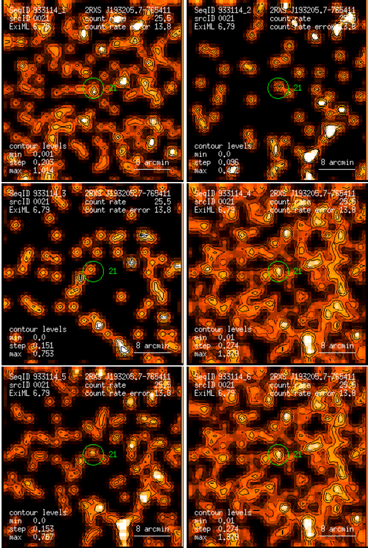
Figure 21: RASS 933114: detection 0021: band rate images, Gaussian filter: (1) PSPC channels 11 – 41, (2) 52 – 90, (3) 91 – 201, (4) 11 – 235, (5) 52 – 201, (6) 11 – 201. Broad band rates in counts/ks. Band rate contour levels in counts/ks/arcmin 2 .
