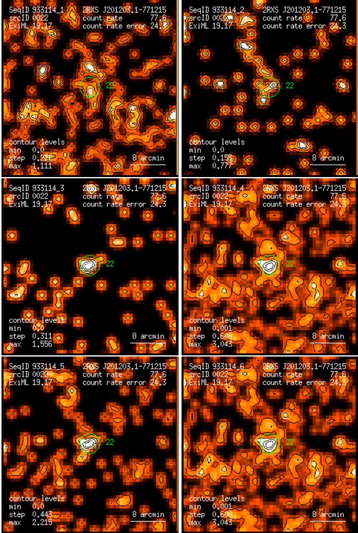
Figure 22: RASS 933114: detection 0022: band rate images, Gaussian filter: (1) PSPC channels 11 – 41, (2) 52 – 90, (3) 91 – 201, (4) 11 – 235, (5) 52 – 201, (6) 11 – 201. Broad band rates in counts/ks. Band rate contour levels in counts/ks/arcmin 2 .
