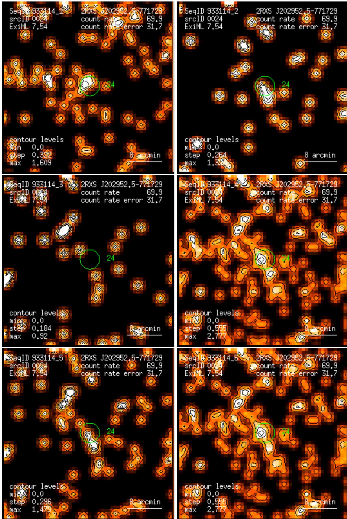
Figure 24: RASS 933114: detection 0024: band rate images, Gaussian filter: (1) PSPC channels 11 – 41, (2) 52 – 90, (3) 91 – 201, (4) 11 – 235, (5) 52 – 201, (6) 11 – 201. Broad band rates in counts/ks. Band rate contour levels in counts/ks/arcmin 2 .
