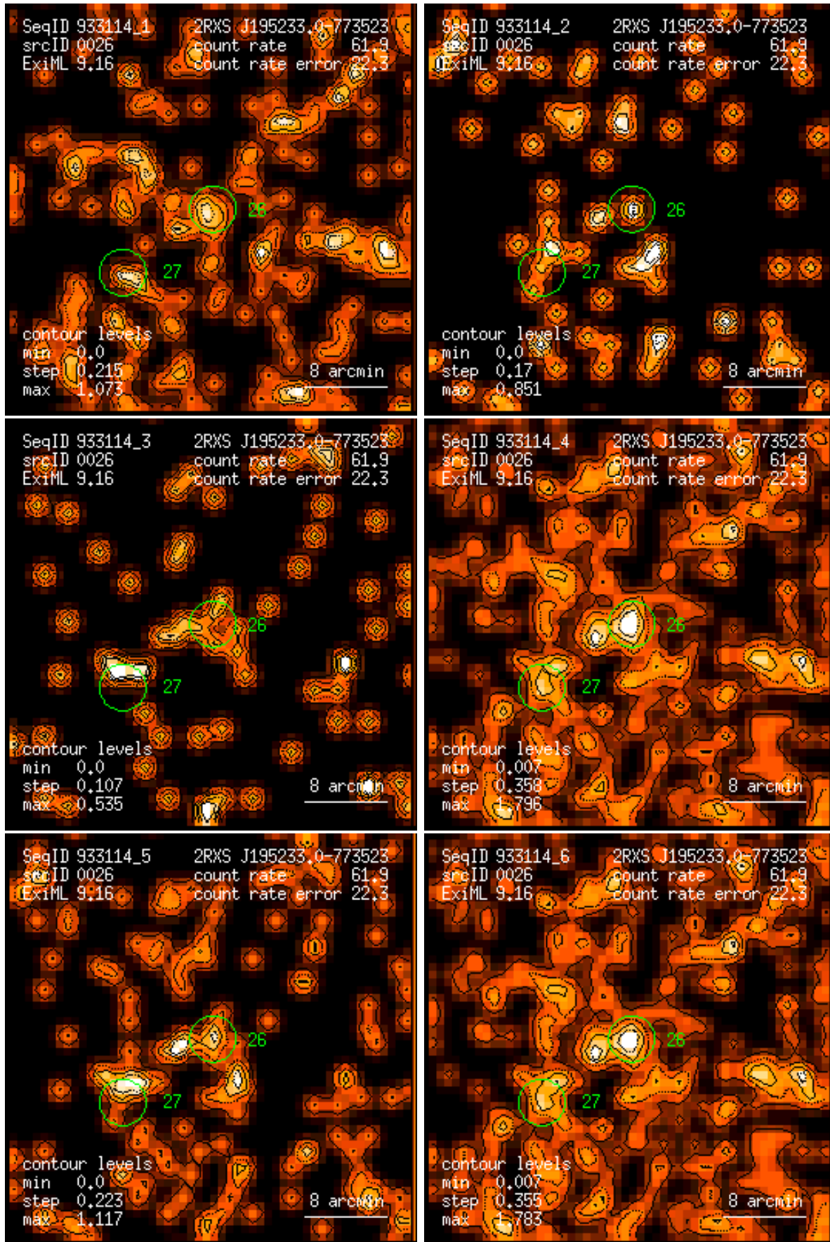
Figure 26: RASS 933114: detection 0026: band rate images, Gaussian filter: (1) PSPC channels 11 – 41, (2) 52 – 90, (3) 91 – 201, (4) 11 – 235, (5) 52 – 201, (6) 11 – 201. Broad band rates in counts/ks. Band rate contour levels in counts/ks/arcmin 2 .
