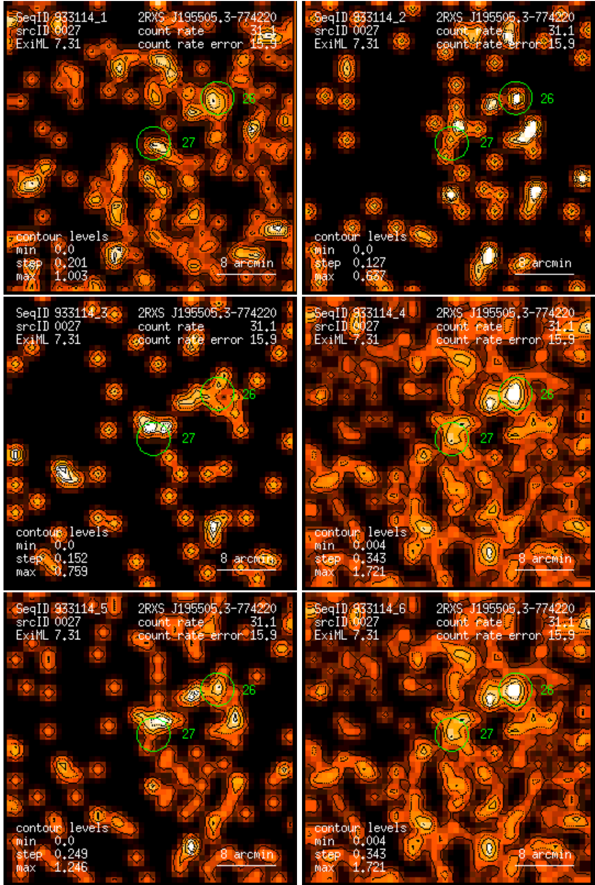
Figure 27: RASS 933114: detection 0027: band rate images, Gaussian filter: (1) PSPC channels 11 – 41, (2) 52 – 90, (3) 91 – 201, (4) 11 – 235, (5) 52 – 201, (6) 11 – 201. Broad band rates in counts/ks. Band rate contour levels in counts/ks/arcmin 2 .
