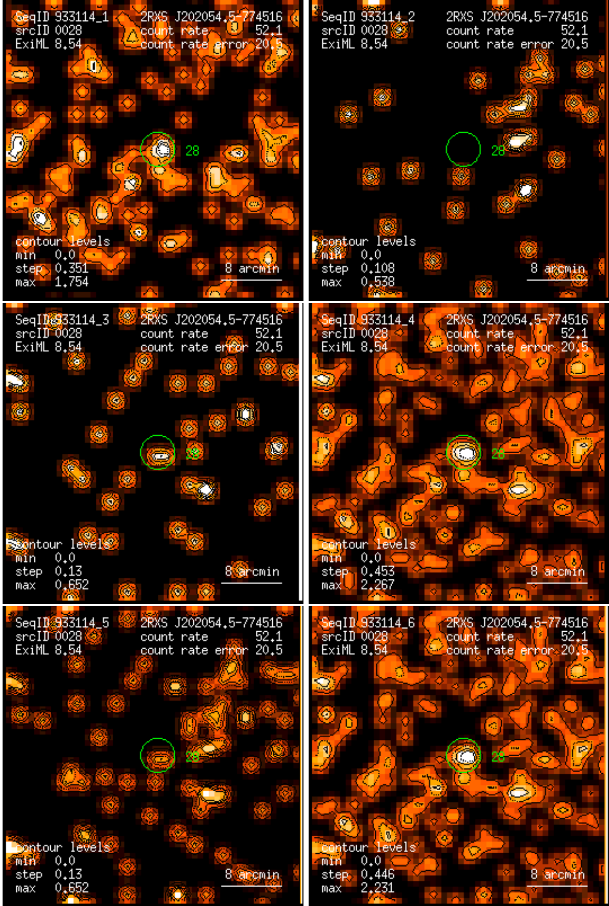
Figure 28: RASS 933114: detection 0028: band rate images, Gaussian filter: (1) PSPC channels 11 – 41, (2) 52 – 90, (3) 91 – 201, (4) 11 – 235, (5) 52 – 201, (6) 11 – 201. Broad band rates in counts/ks. Band rate contour levels in counts/ks/arcmin 2 .
