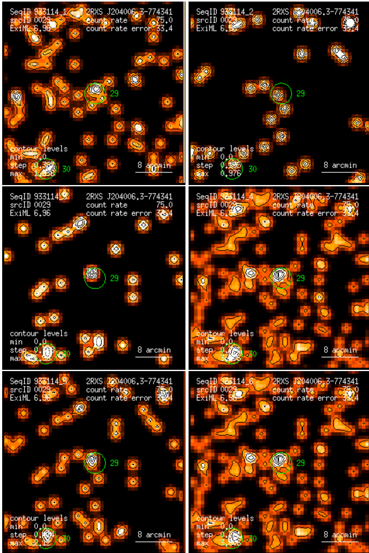
Figure 29: RASS 933114: detection 0029: band rate images, Gaussian filter: (1) PSPC channels 11 – 41, (2) 52 – 90, (3) 91 – 201, (4) 11 – 235, (5) 52 – 201, (6) 11 – 201. Broad band rates in counts/ks. Band rate contour levels in counts/ks/arcmin 2 .
