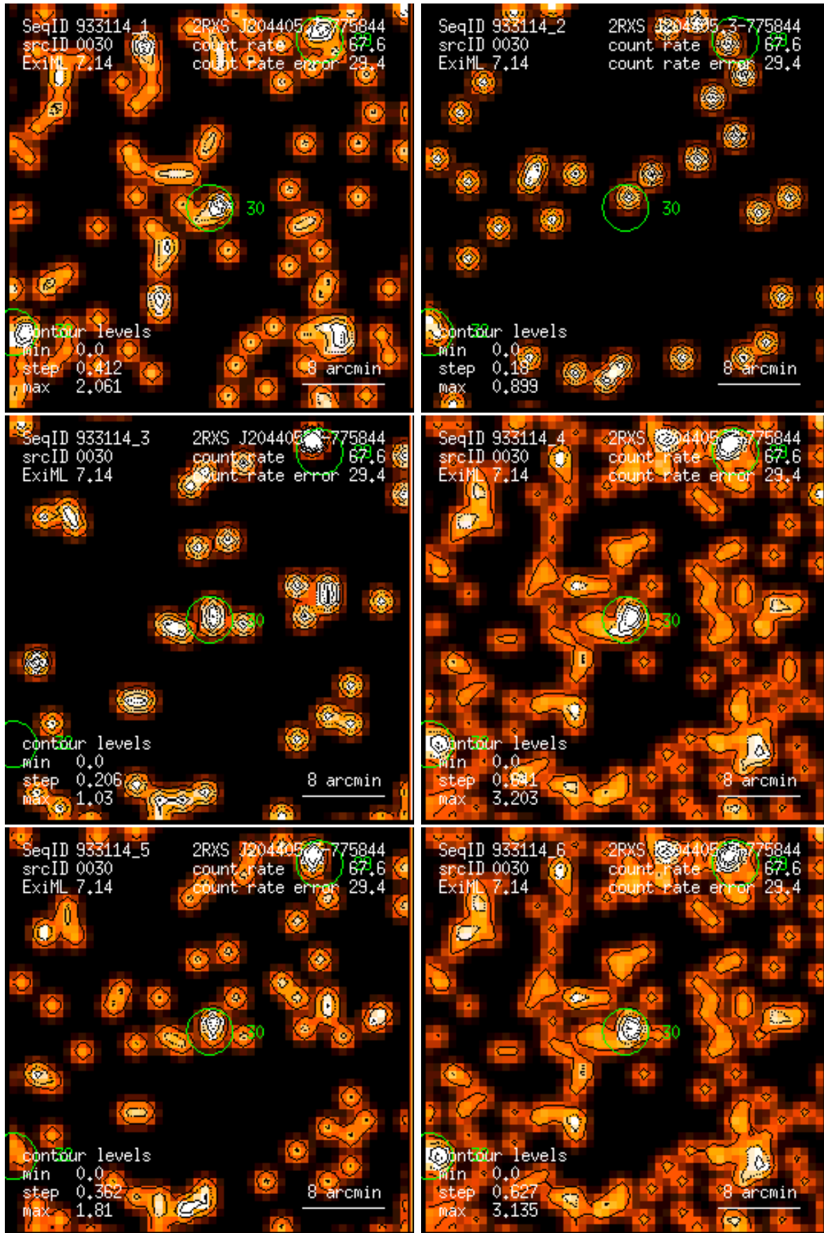
Figure 30: RASS 933114: detection 0030: band rate images, Gaussian filter: (1) PSPC channels 11 – 41, (2) 52 – 90, (3) 91 – 201, (4) 11 – 235, (5) 52 – 201, (6) 11 – 201. Broad band rates in counts/ks. Band rate contour levels in counts/ks/arcmin 2 .
