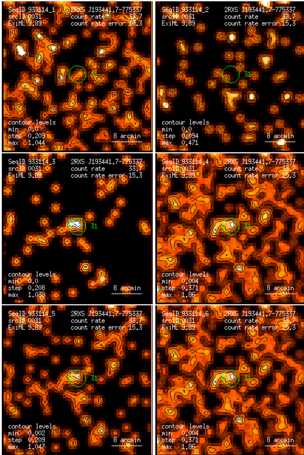
Figure 31: RASS 933114: detection 0031: band rate images, Gaussian filter: (1) PSPC channels 11 – 41, (2) 52 – 90, (3) 91 – 201, (4) 11 – 235, (5) 52 – 201, (6) 11 – 201. Broad band rates in counts/ks. Band rate contour levels in counts/ks/arcmin 2 .
