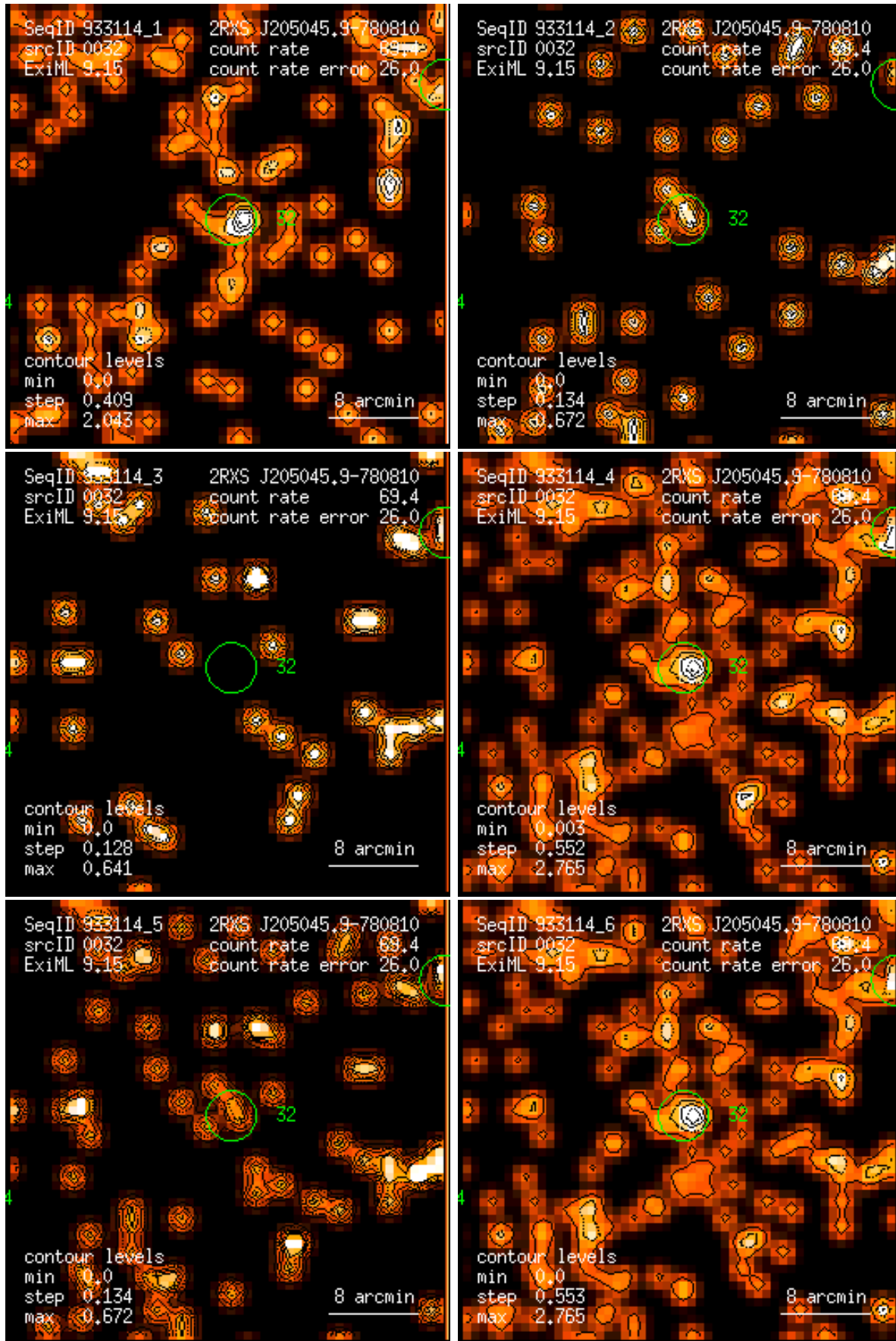
Figure 32: RASS 933114: detection 0032: band rate images, Gaussian filter: (1) PSPC channels 11 – 41, (2) 52 – 90, (3) 91 – 201, (4) 11 – 235, (5) 52 – 201, (6) 11 – 201. Broad band rates in counts/ks. Band rate contour levels in counts/ks/arcmin 2 .
