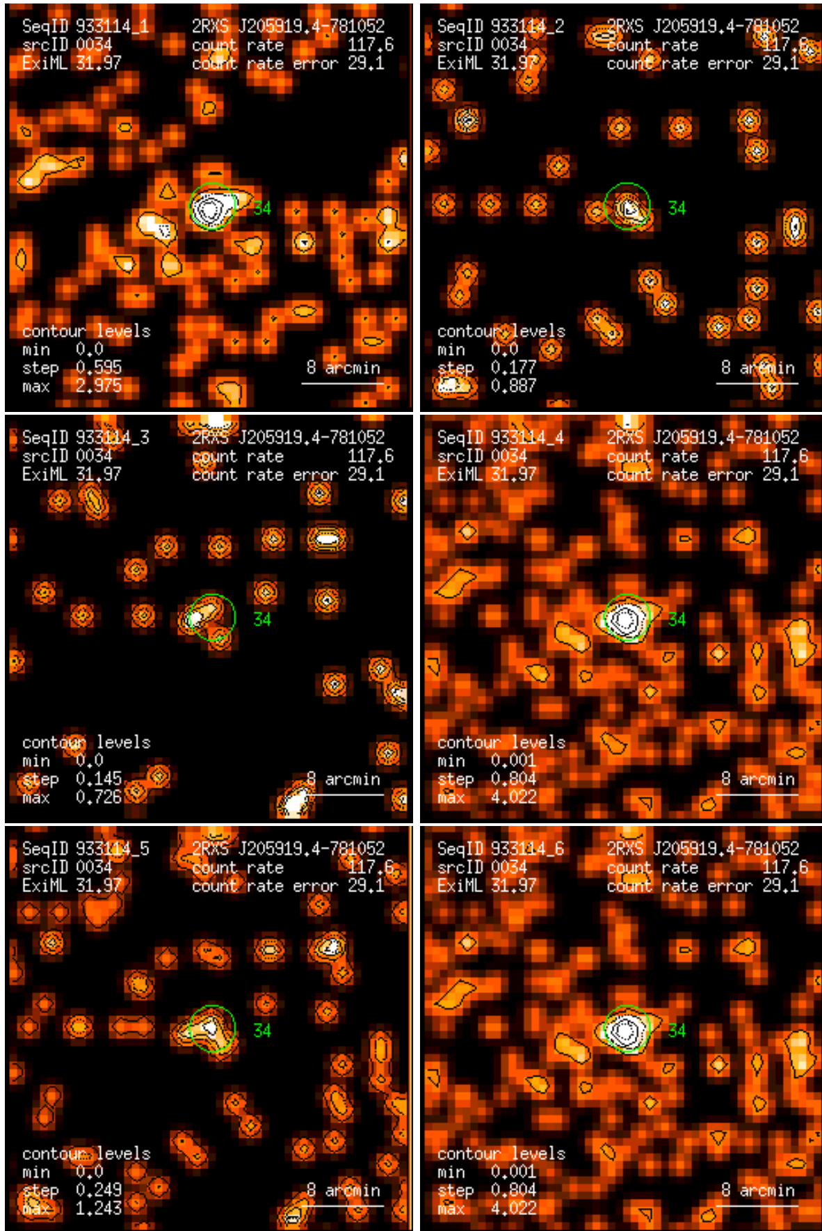
Figure 34: RASS 933114: detection 0034: band rate images, Gaussian filter: (1) PSPC channels 11 – 41, (2) 52 – 90, (3) 91 – 201, (4) 11 – 235, (5) 52 – 201, (6) 11 – 201. Broad band rates in counts/ks. Band rate contour levels in counts/ks/arcmin 2 .
