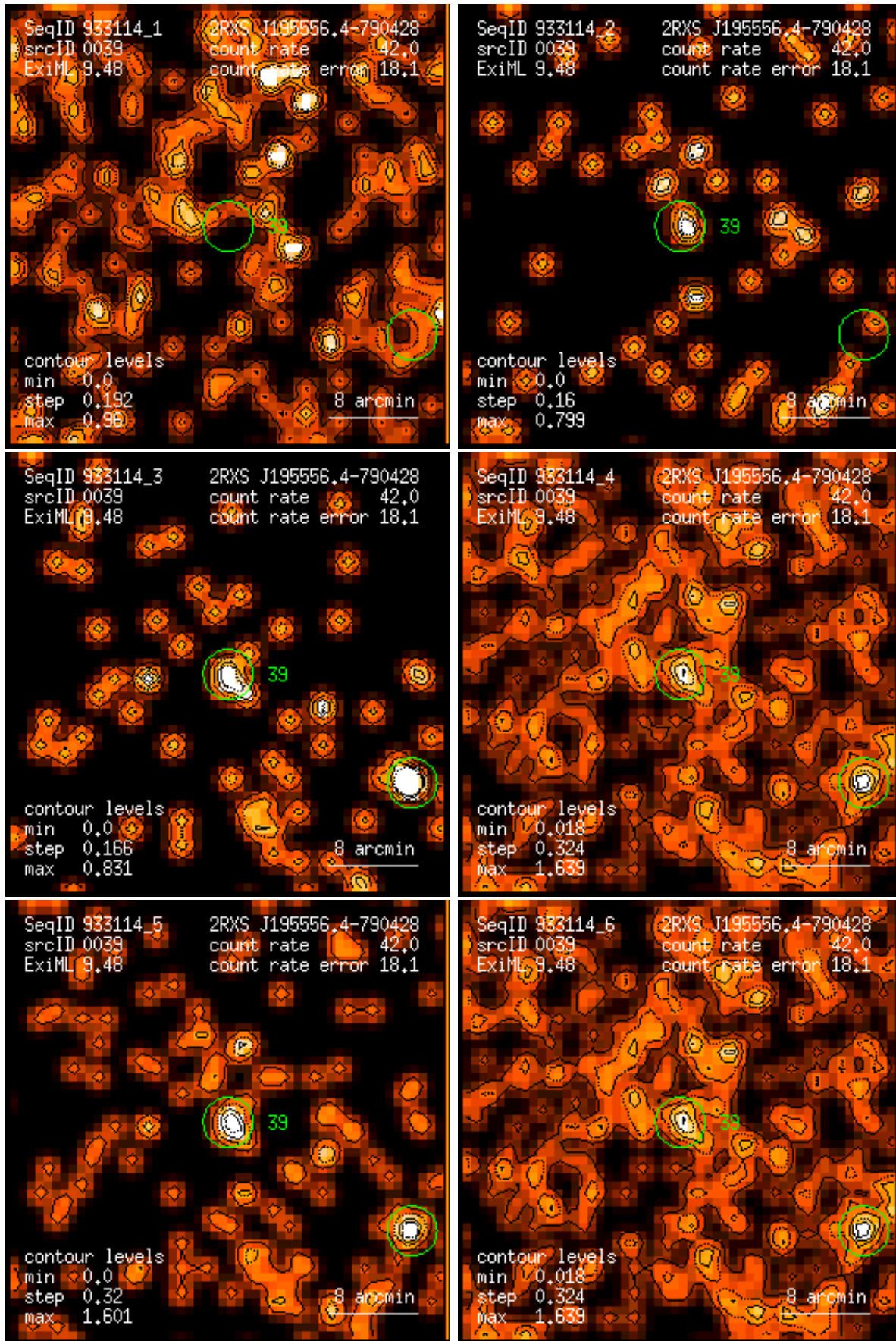
Figure 39: RASS 933114: detection 0039: band rate images, Gaussian filter: (1) PSPC channels 11 – 41, (2) 52 – 90, (3) 91 – 201, (4) 11 – 235, (5) 52 – 201, (6) 11 – 201. Broad band rates in counts/ks. Band rate contour levels in counts/ks/arcmin 2 .
