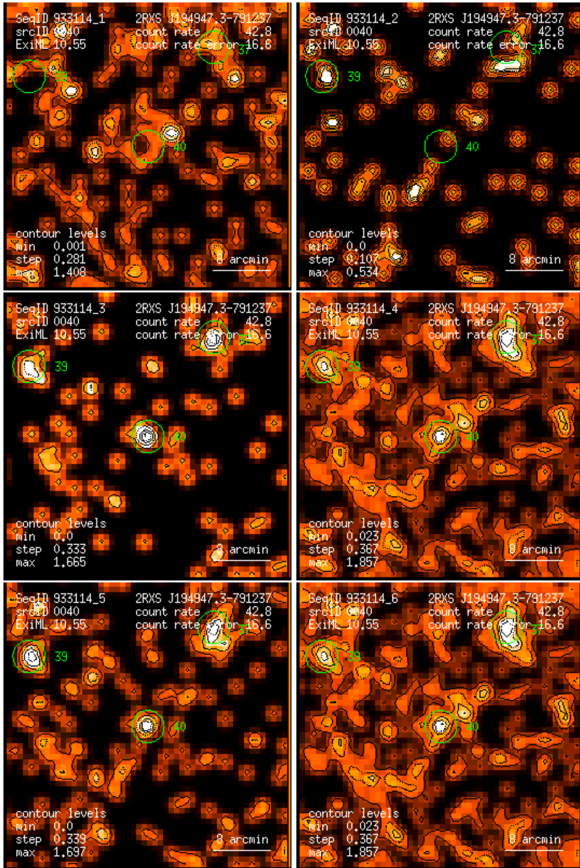
Figure 40: RASS 933114: detection 0040: band rate images, Gaussian filter: (1) PSPC channels 11 – 41, (2) 52 – 90, (3) 91 – 201, (4) 11 – 235, (5) 52 – 201, (6) 11 – 201. Broad band rates in counts/ks. Band rate contour levels in counts/ks/arcmin 2 .
