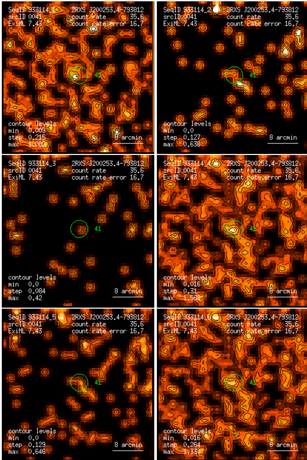
Figure 41: RASS 933114: detection 0041: band rate images, Gaussian filter: (1) PSPC channels 11 – 41, (2) 52 – 90, (3) 91 – 201, (4) 11 – 235, (5) 52 – 201, (6) 11 – 201. Broad band rates in counts/ks. Band rate contour levels in counts/ks/arcmin 2 .
