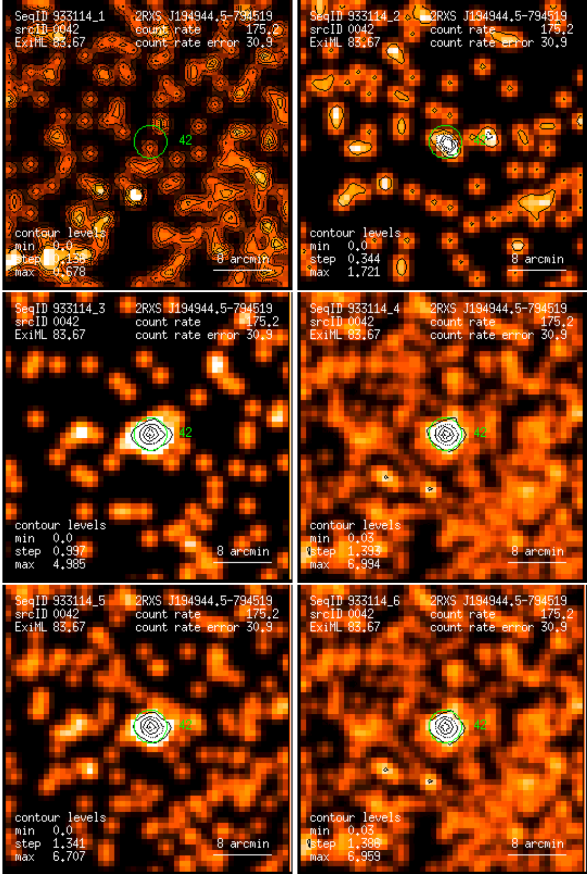
Figure 42: RASS 933114: detection 0042: band rate images, Gaussian filter: (1) PSPC channels 11 – 41, (2) 52 – 90, (3) 91 – 201, (4) 11 – 235, (5) 52 – 201, (6) 11 – 201. Broad band rates in counts/ks. Band rate contour levels in counts/ks/arcmin 2 .
