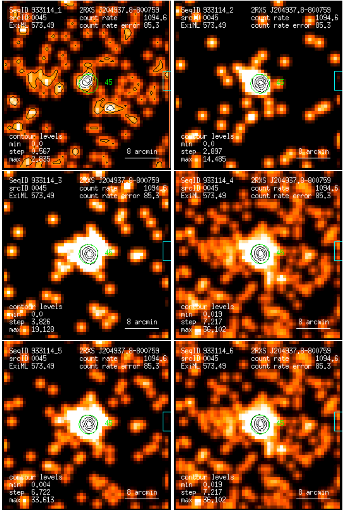
Figure 45: RASS 933114: detection 0045: band rate images, Gaussian filter: (1) PSPC channels 11 – 41, (2) 52 – 90, (3) 91 – 201, (4) 11 – 235, (5) 52 – 201, (6) 11 – 201. Broad band rates in counts/ks. Band rate contour levels in counts/ks/arcmin 2 .
