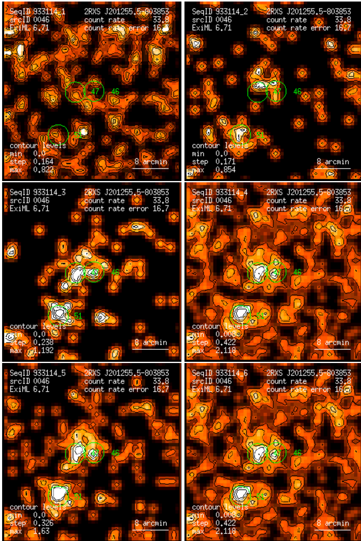
Figure 46: RASS 933114: detection 0046: band rate images, Gaussian filter: (1) PSPC channels 11 – 41, (2) 52 – 90, (3) 91 – 201, (4) 11 – 235, (5) 52 – 201, (6) 11 – 201. Broad band rates in counts/ks. Band rate contour levels in counts/ks/arcmin 2 .
