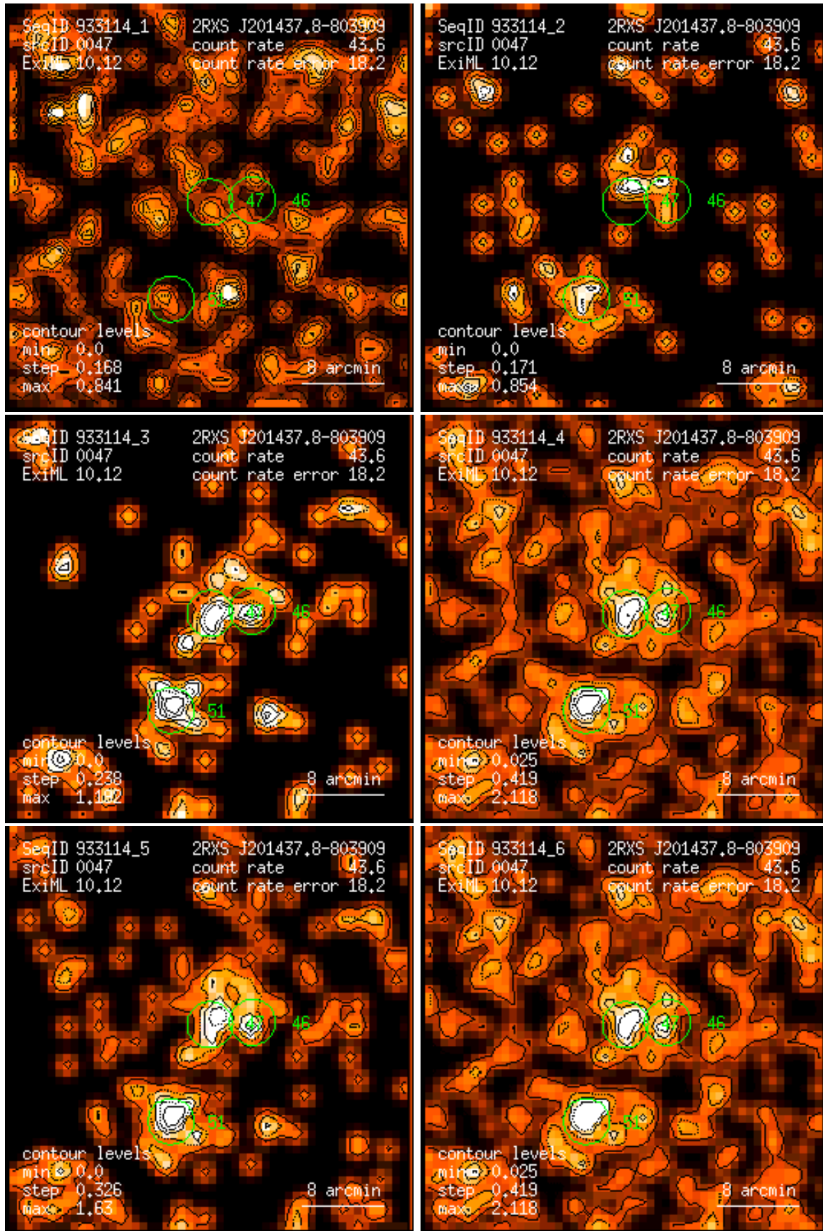
Figure 47: RASS 933114: detection 0047: band rate images, Gaussian filter: (1) PSPC channels 11 – 41, (2) 52 – 90, (3) 91 – 201, (4) 11 – 235, (5) 52 – 201, (6) 11 – 201. Broad band rates in counts/ks. Band rate contour levels in counts/ks/arcmin 2 .
