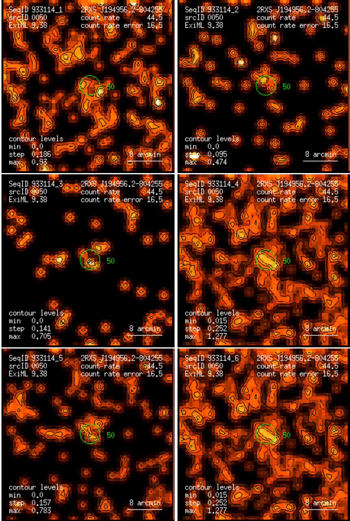
Figure 50: RASS 933114: detection 0050: band rate images, Gaussian filter: (1) PSPC channels 11 – 41, (2) 52 – 90, (3) 91 – 201, (4) 11 – 235, (5) 52 – 201, (6) 11 – 201. Broad band rates in counts/ks. Band rate contour levels in counts/ks/arcmin 2 .
