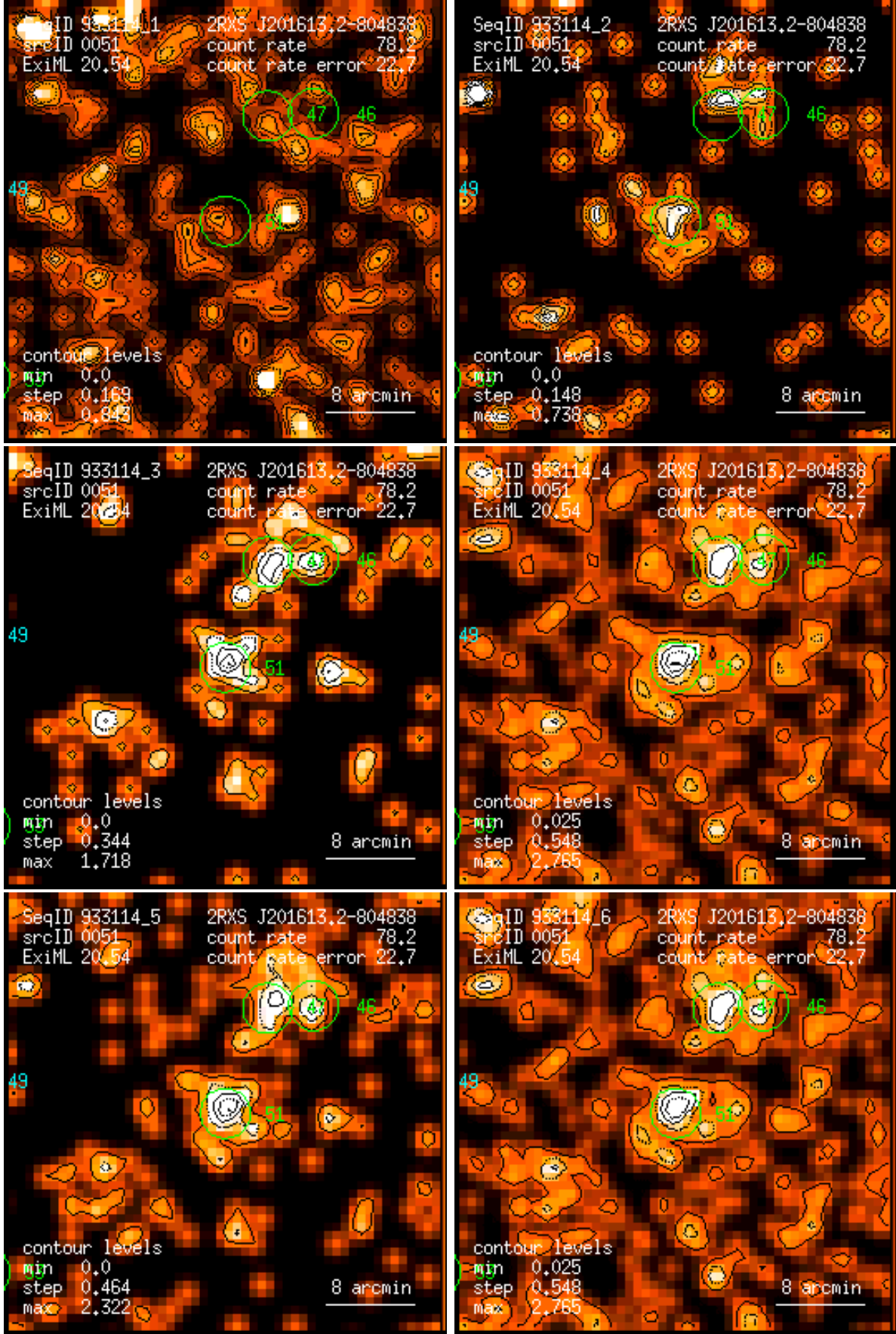
Figure 51: RASS 933114: detection 0051: band rate images, Gaussian filter: (1) PSPPC channels 11 – 41, (2) 52 – 90, (3) 91 – 201, (4) 11 – 235, (5) 52 – 201, (6) 11 – 201. Broad band rates in counts/ks. Band rate contour levels in counts/ks/arcmin 2 .
